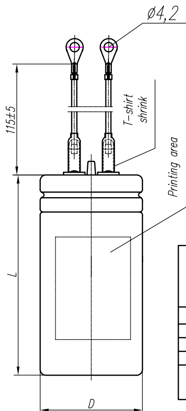
Capacitor dimensions
