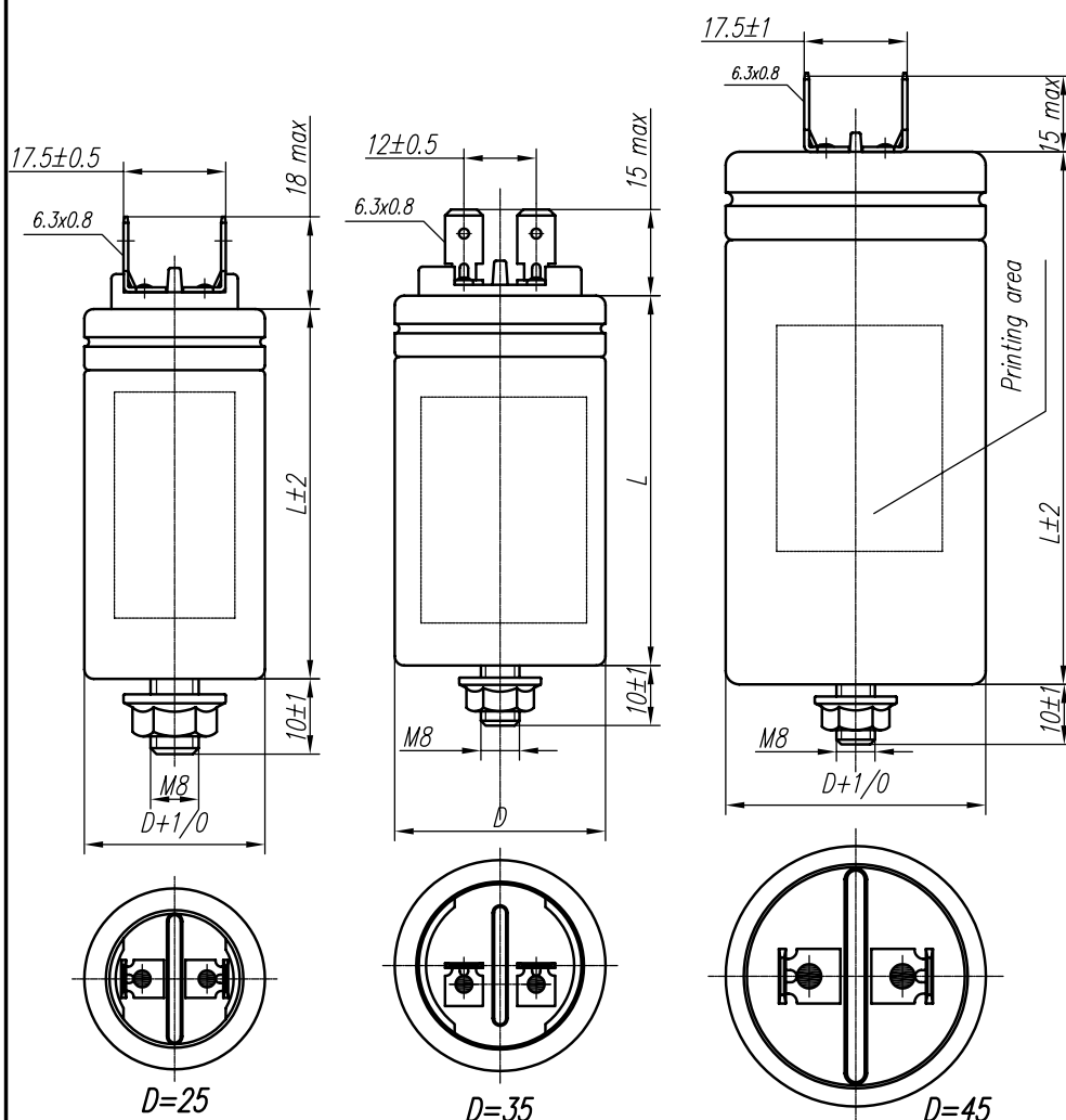
Capacitor dimensions
